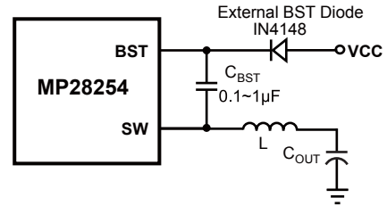
Figure 8—Add Optional External Bootstrap Diode to Enhance Efficiency
